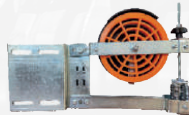
Elevator Speed Governor Bottom Tension Pulley
